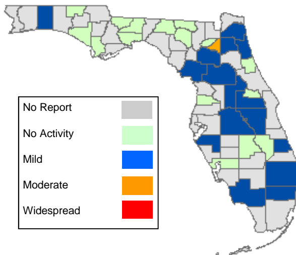
Map 2: Weekly County Influenza Activity for Week 27 as Reported by 11:00 a.m. July 11, 2012
